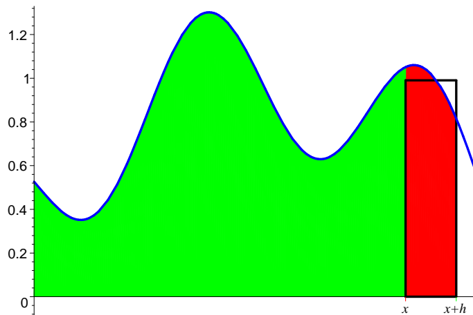
F(x) = grüne Fläche, F(x+h) - F(x) = rote Fläche
